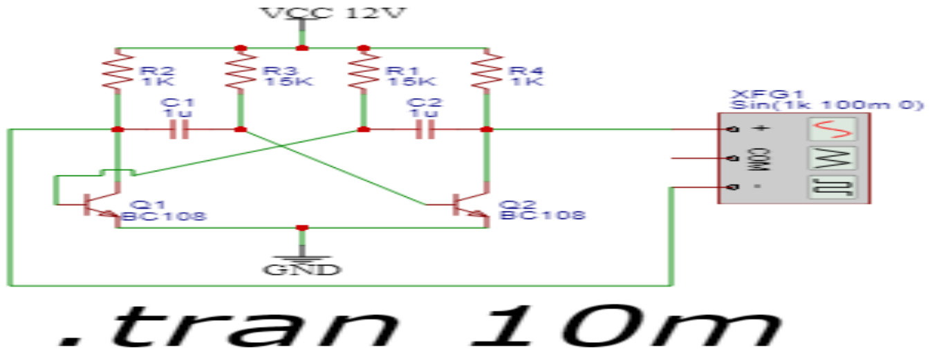
Figure 4. The circuit diagram of the Astable Multivibrator Oscillator.
