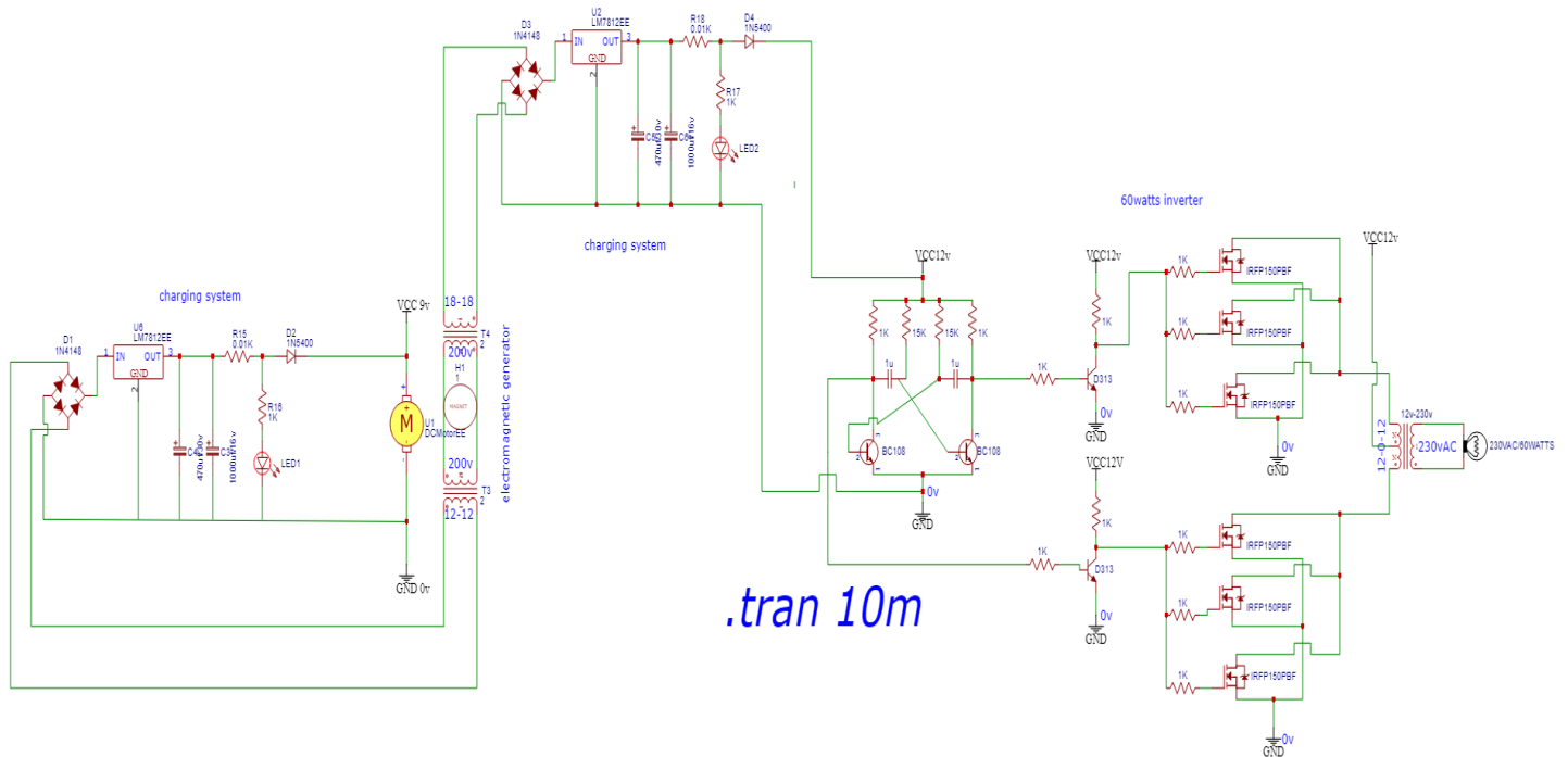
Figure 9. Circuit diagram of electromagnetic DC generator powered single phase voltage source 60watts inverter.
