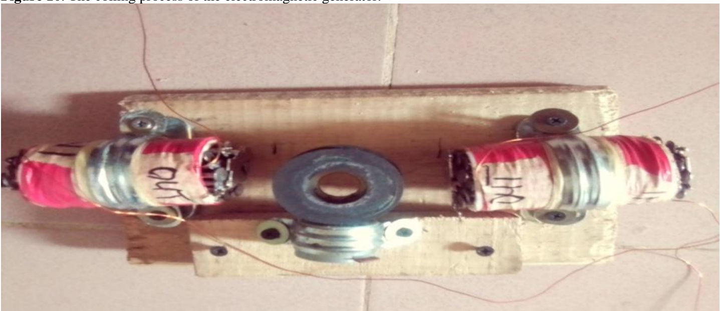
Figure 11. Assembling of the electromagnetic DC generator system.
