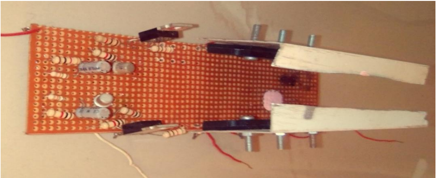
Figure 12. Astable multivibrator and power switching MOSFETS
