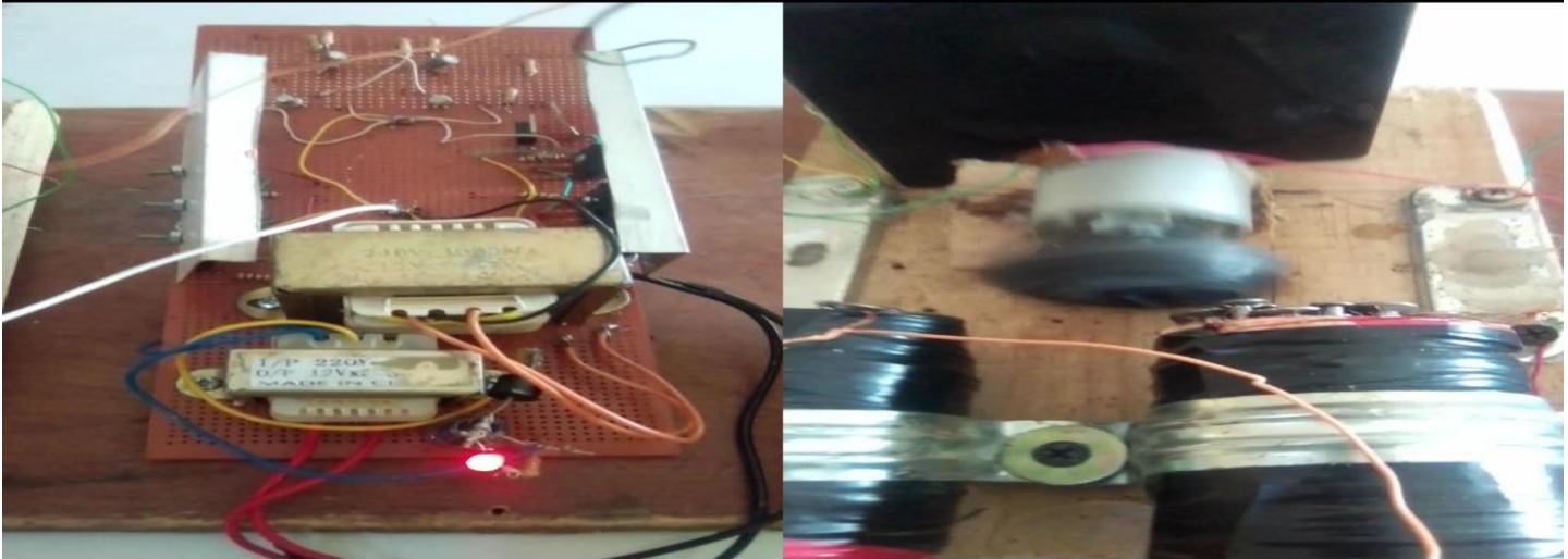
Figure 14. Testing of the electromagnetic DC generator powered inverter system
