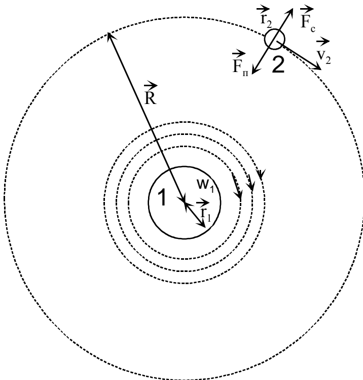
Fig. 1. Two-dimensional model of gravitational interaction of two bodies. Forces operating on a body 2 are specified. The F_c -centrifugal force, F_n -force of an attraction of a body 2 from a body 1, v_2 – the linear speed of a body 2 on an orbit, R – the radius of an orbit, r_1 – the radius of a body 1, r_2 – the radius of a body 2, w_1 – the angular speed of rotation of air on a surface of a body 1, m_2 – body weight 2.
